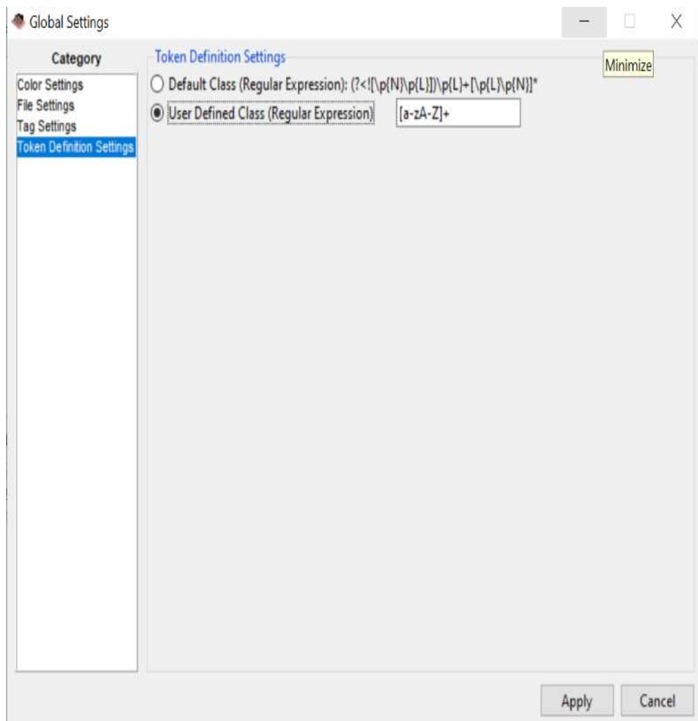
Figure 3.5. Setting up the Token definition
