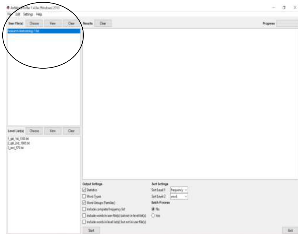
Figure 3.4. An interface of AntWordProfiler
