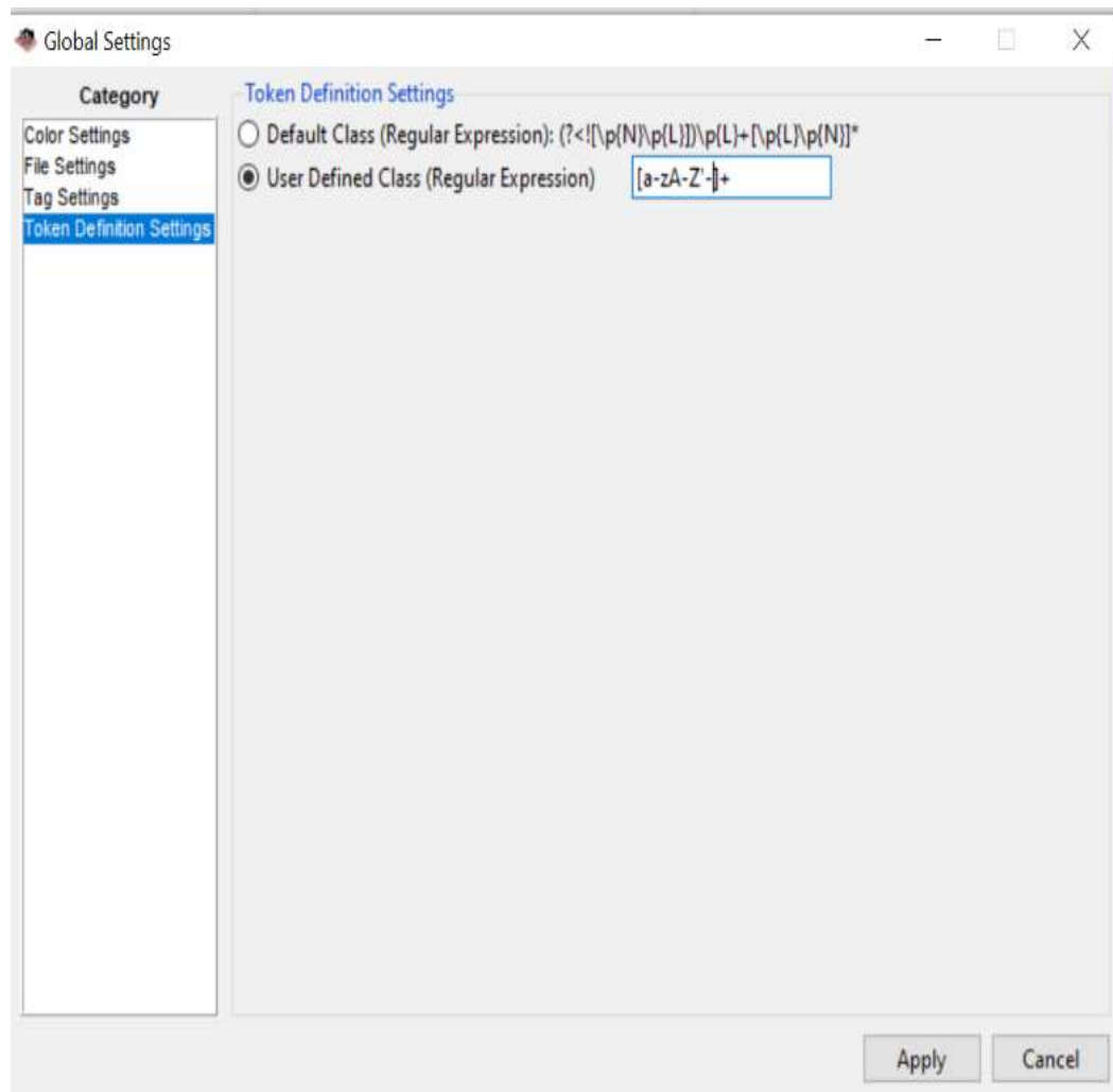
Figure 3.6. Setting up the 'Token definition' add the characters
