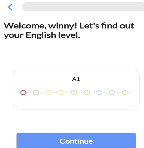
Figure 2.8 AI Test
